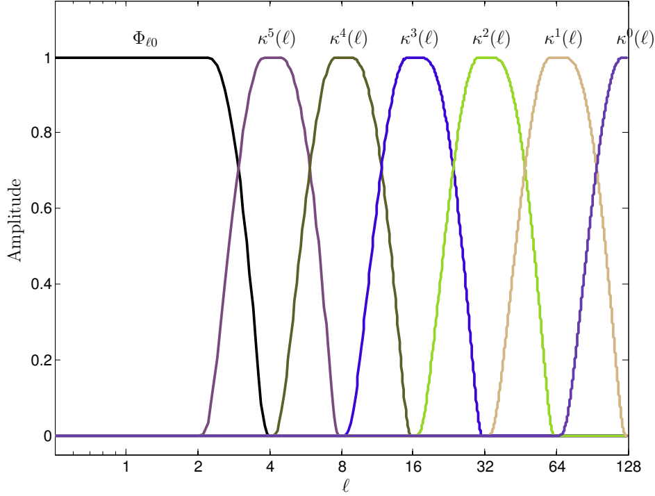
Figure 1: Scale-discretised wavelet tiling in harmonic space ( L = 128 , \lambda = 2 , N = 3 , J = 5 ).
