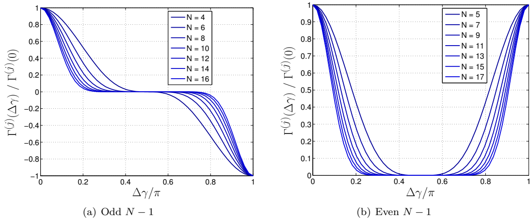
Figure 4: Directional auto-correlation for even and odd N - 1 . As N increases the directional auto-correlation function becomes more peaked and the associated wavelet more directional.
