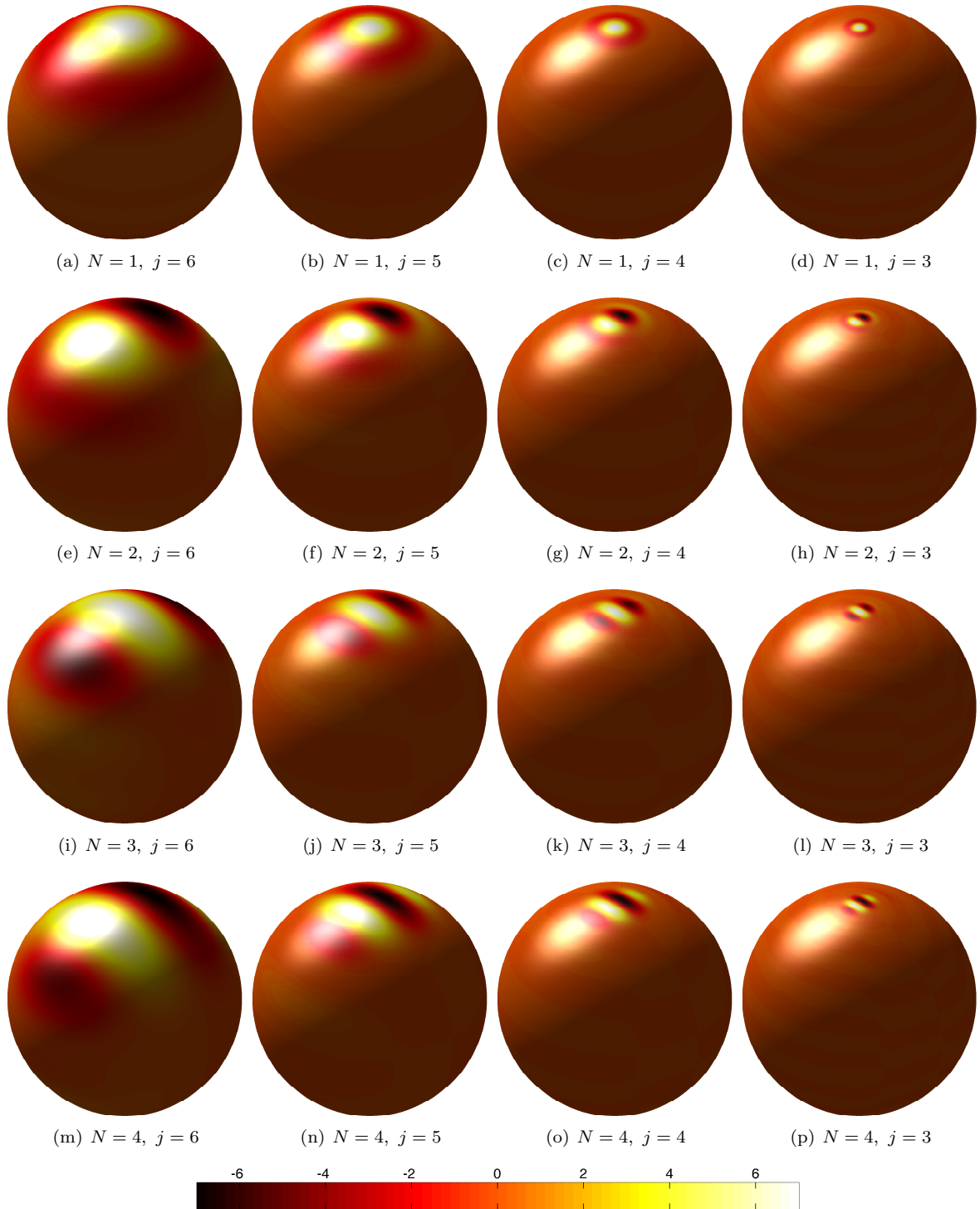
Figure 3: Directional scale-discretised wavelets ( L = 256 , \lambda = 2 , J = 8 ). Wavelet scale j varies across columns, while azimuthal band-limit N values across rows.
